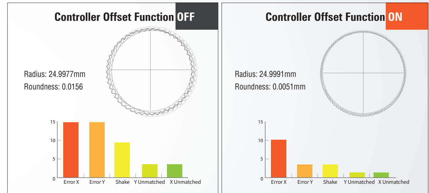
Circuit Function Verification Result: (Diameter 50mm, Speed: 400mm/min)
